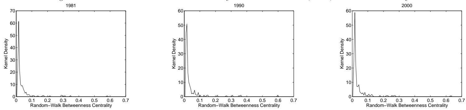
Figure 15: Random Walk Betweenness Centrality distributions in 1981, 1990, 2000: Kernel density estimates.
