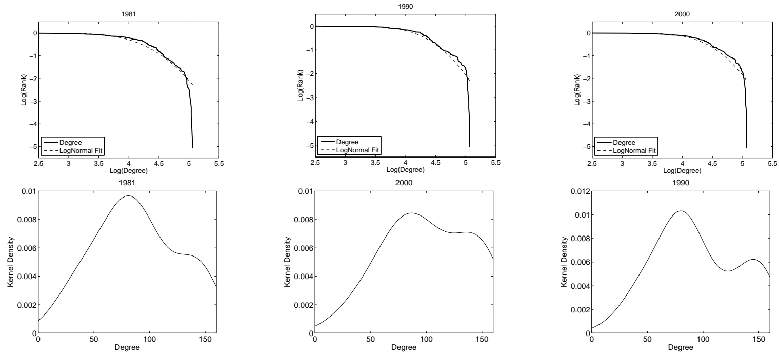
Figure 2: The WTW as a BUN. Degree distributions in 1981, 1990, 2000. Top panels: Size-rank plots (dashed line: lognormal fit). Bottom panels: Kernel density estimates.
