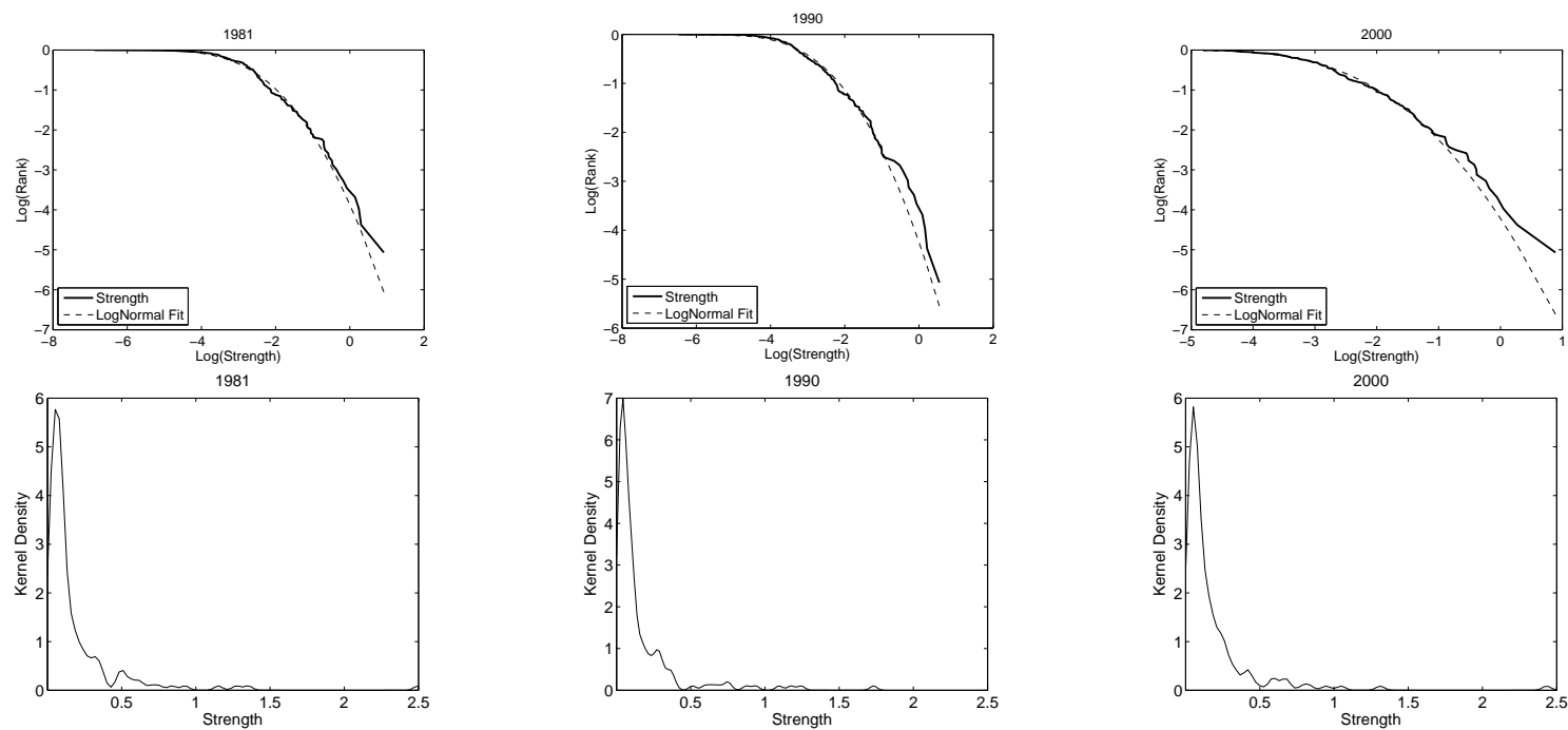
Figure 4: The WTW as a WUN. Strength distributions in 1981, 1990, 2000. Top panels: Size-rank plots (dashed line: lognormal fit). Bottom panels: Kernel density estimates.
